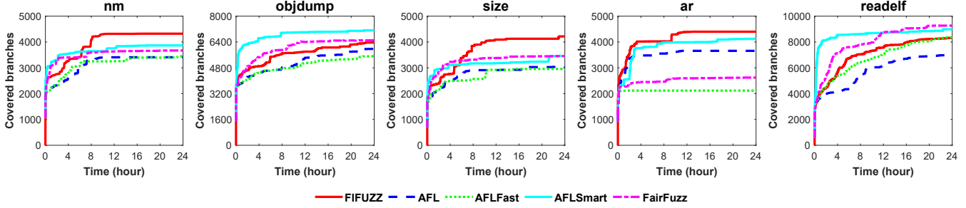
Figure 13: Code coverage of FIFUZZ and the four fuzzing tools.
