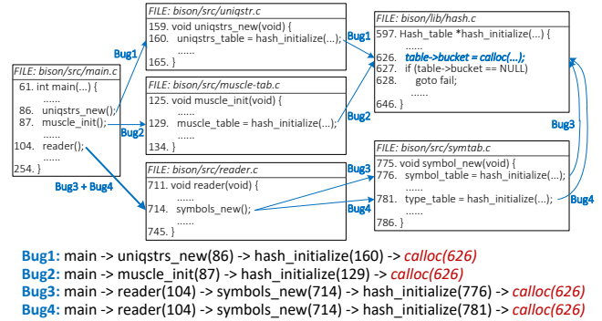
Figure 11: Example bugs caused by the same error site.
