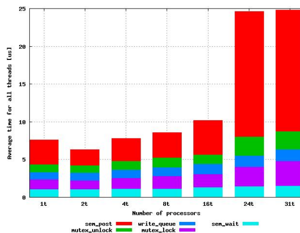
Figure 10. Distribution of execution time for the submit_mb in dynamic scheduling with tail-submit.
