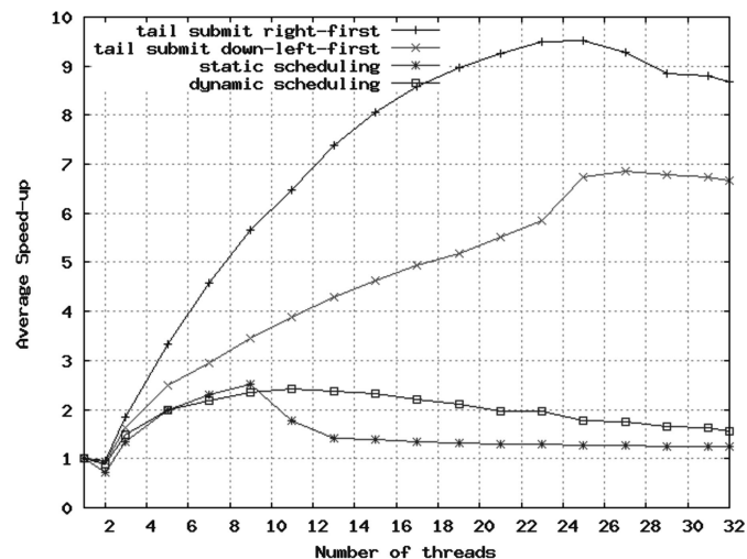
Figure 5. Speedup using Different Scheduling Approaches.
