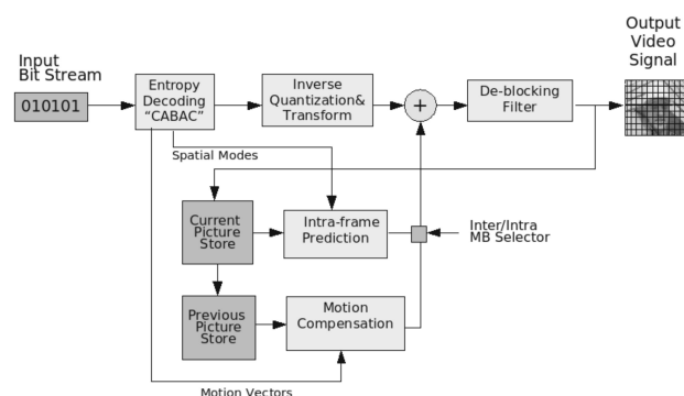
Figure 1. Block diagram of the H.264 decoding process.
